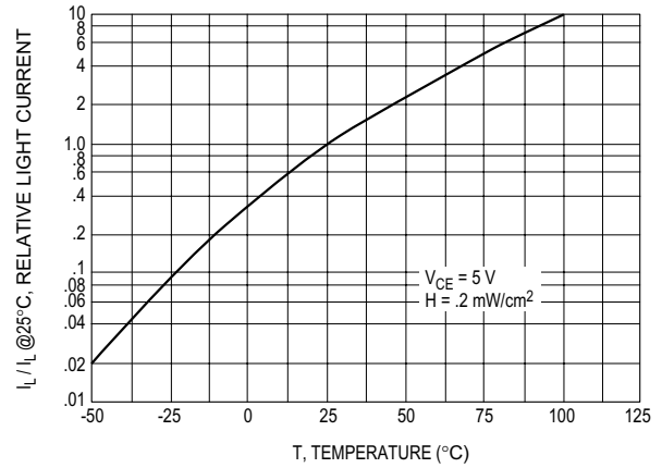
Figure 2. Relative Light Current vs. Ambient Temperature
