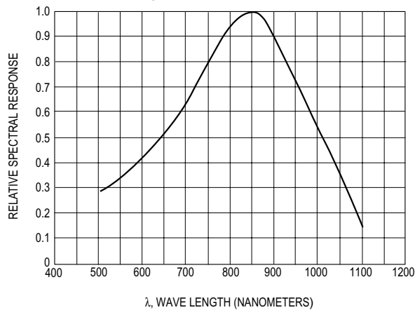
Figure 3. Spectral Response
