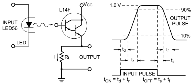
Figure 5. Test Circuit and Voltage Waveforms
