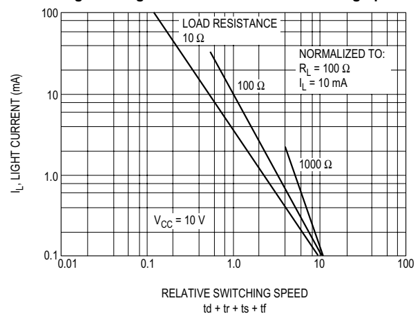
Figure 6. Light Current vs. Relative Switching Speed
