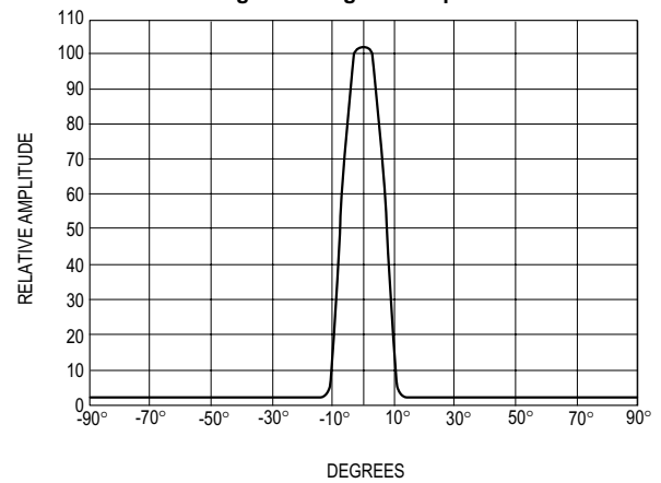
Figure 4. Angular Response
