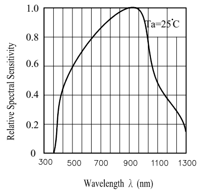
Fig.5 Spectral Sensitivity
